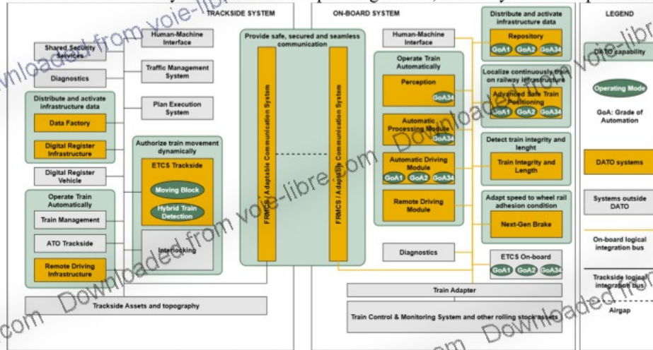
Fig. 2. DATO technical configurations' view
